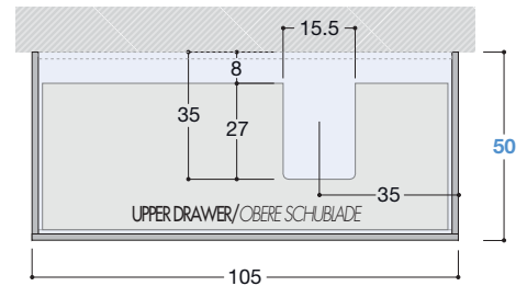
Plan view D.50 / Grundriss T.50
