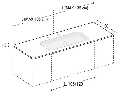
BASIN D / BECKEN D
