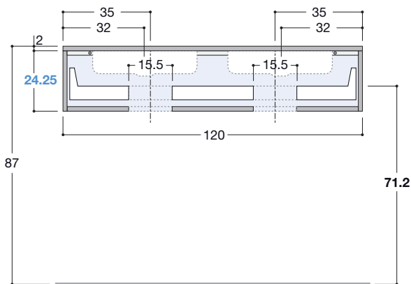
Front view / Frontansicht
