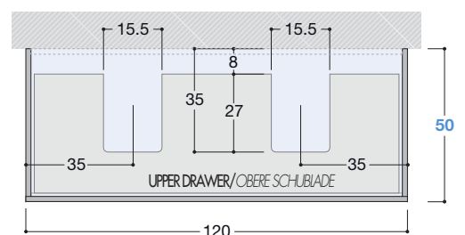
Plan view D.50 / Grundriss T.50
