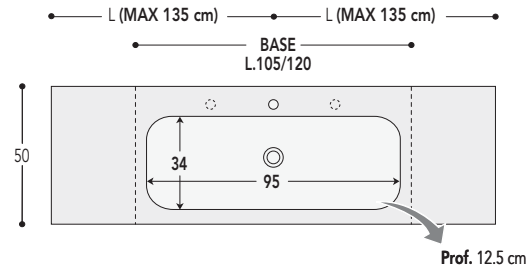
BASIN D / BECKEN D
