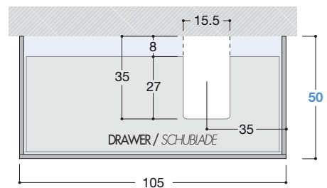
Plan view D.50 / Grundriss T.50
