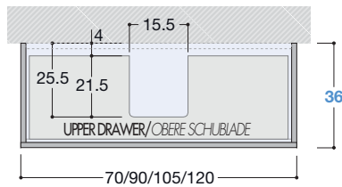
Plan view D.36 / Grundriss T.36
