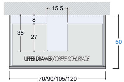
Plan view D.50 / Grundriss T.50
